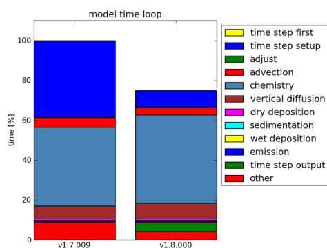
Figure 17-5 Run time spent on processes for v1.7.009 and v1.8.000 . Note that for v1.7.009 the 'time step output' task was included in the 'other' task.
